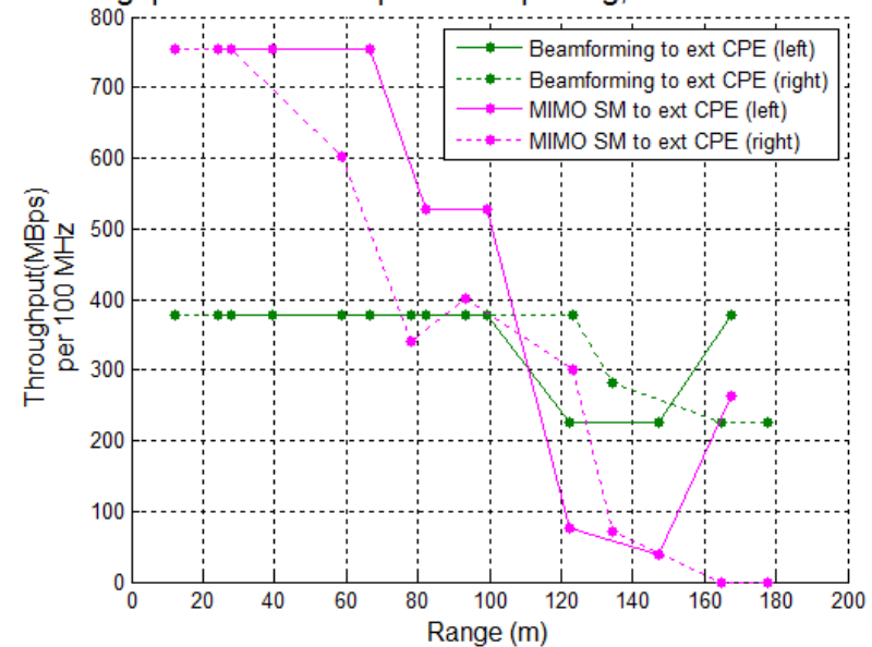
Throughput with MIMO Spatial Multiplexing, Exterior Window CPE
