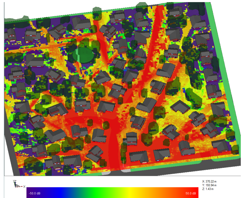
SINR w/MIMO Beamforming
