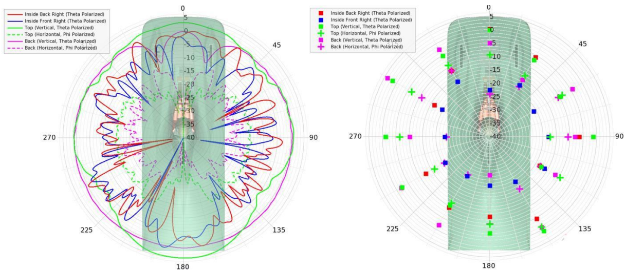
Fig. 5. XY slice of realized gain from modeling (A) and normalized average power from experimental measurements (B).
