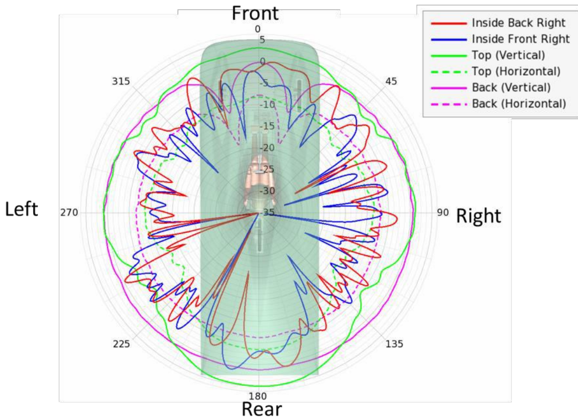
Fig. 2. XY cut of a theta-polarized realized gain plot for six antenna positions.
