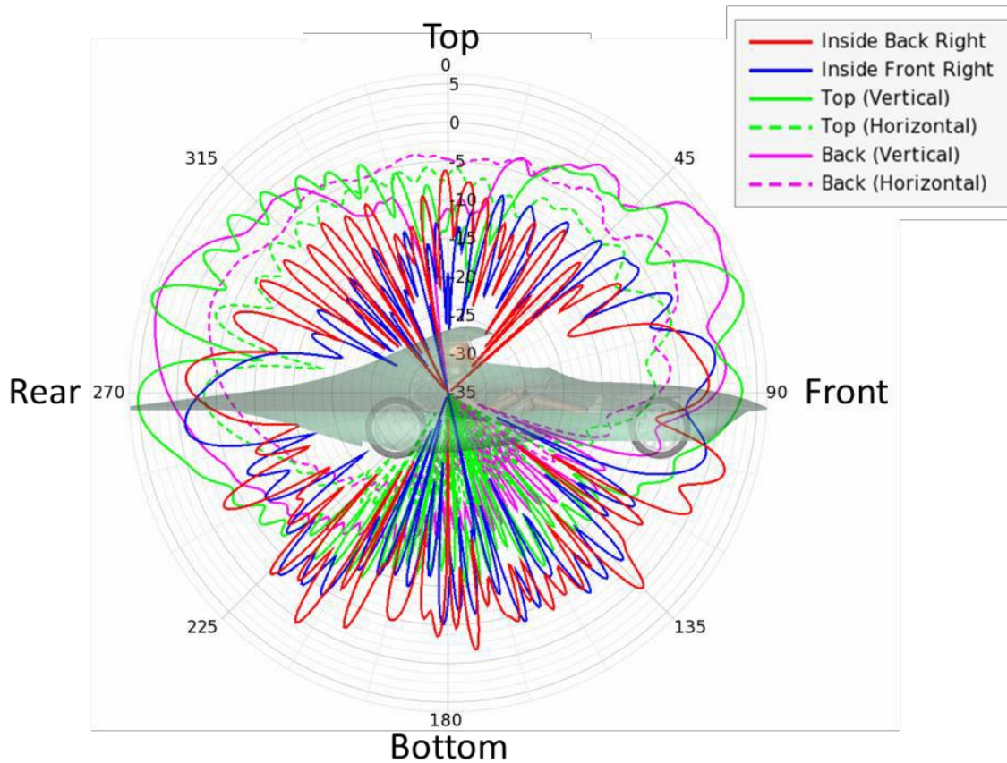
Fig. 3. YZ slice of theta-polarized realized gain plot for the six antenna positions.
