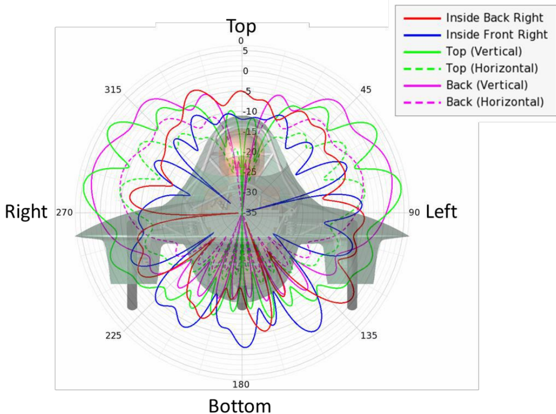
Fig. 4. XZ slice of theta-polarized realized gain plot for the six antenna positions.
