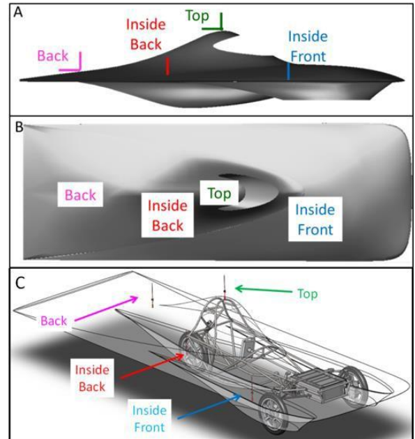
Fig. 1. Locations of antenna in and on the solar vehicle body. Positions “Inside Back” and “Inside Front” are inside the body and are both vertical antennas. Positions “Top” and “Back” are outside and are analyzed for both vertical and horizontal antennas. Colors of the numbers in this figure correlate to the colors of the lines in Figures 2, 3, and 4.
