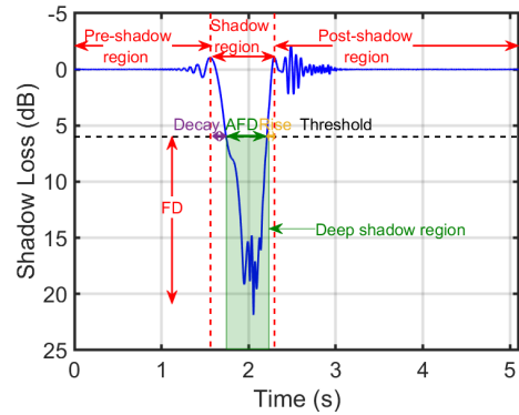
FIGURE 2. Typical parameters used to characterize human shadowing, overlaid on a sample measured signal profile (blue).
